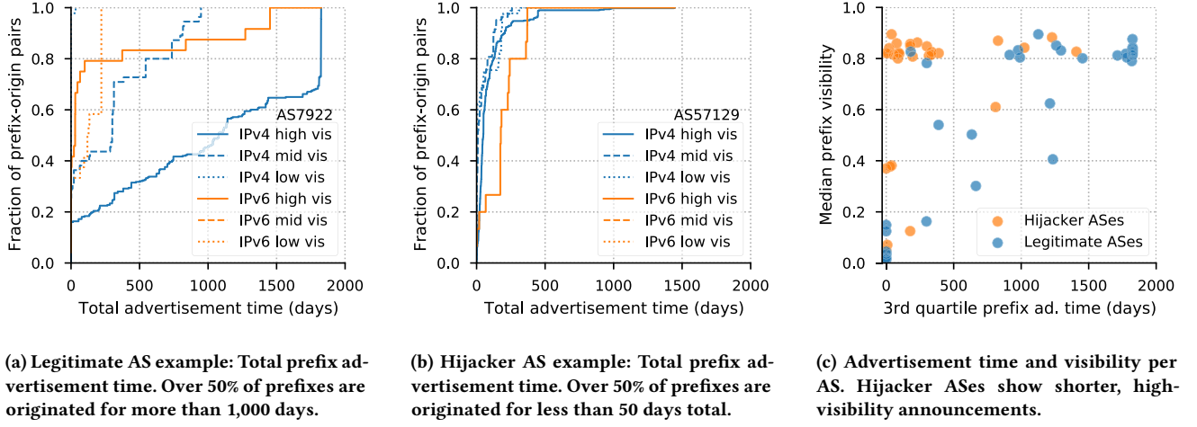
Figure 5: Advertisement longevity and visibility of prefixes originated by legitimate and serial hijacker ASes.
