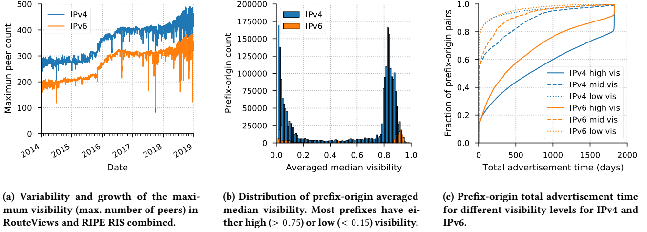
Figure 2: Visibility of prefix-origin pairs in the global routing table.
