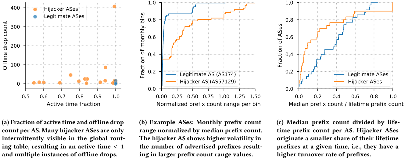
Figure 4: Volatility metrics of prefix origination behavior for serial hijackers and legitimate ASes.
